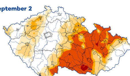
State of soil drought in the surface layer of 0–40 cm on April 23, July 7, August 28 and September 2, 2025.
