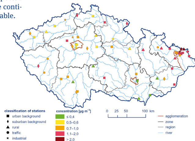
Annual average concentrations of benzo[a]pyrene in the Czech Republic, 2015–2025.
