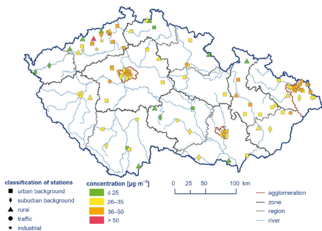
36 th highest 24-hour average PM 10 concentration at AIM monitoring stations, 2025.
